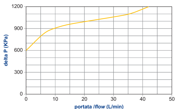
BY-PASS / BY-PASS
